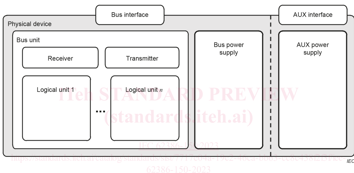
Figure 2 – AUX power supply combined with a bus unit and a bus power supply
