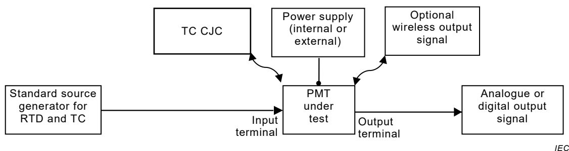
Figure 1 – Schematic example of test set-up for temperature measurement transmitters
