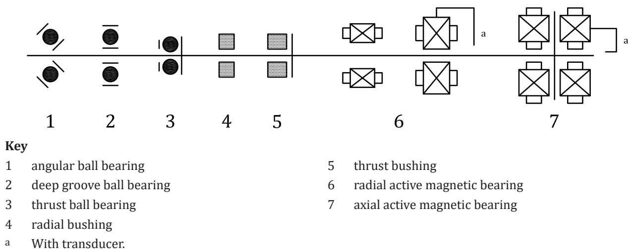
Figure 1 — Graphical symbols for bearings
